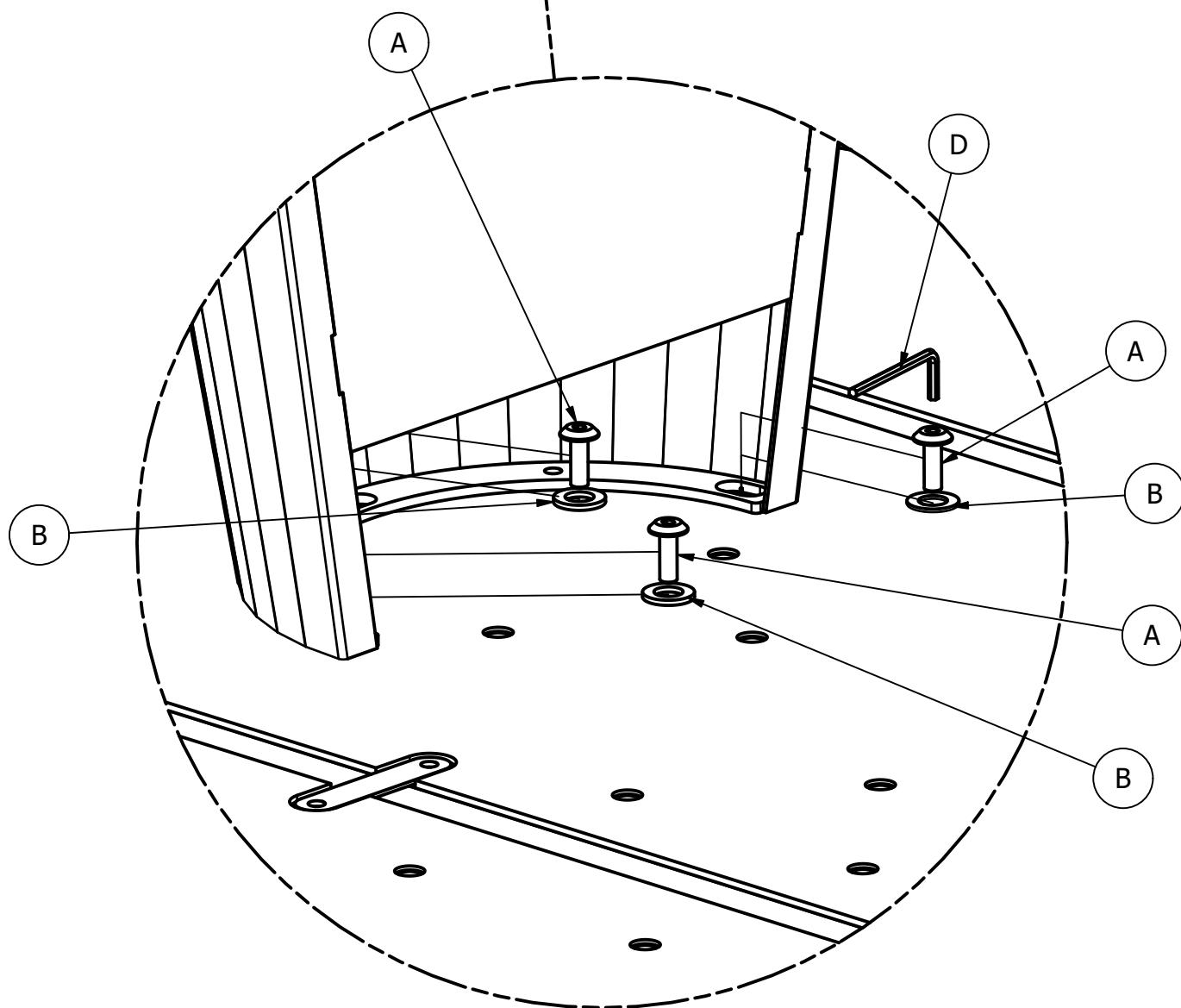
DETAIL a
