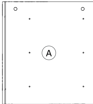
FI09913 484x442x30mm
