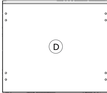
BA02523 520x444x30mm
