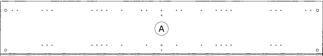
FI9632 2074x353x38mm
