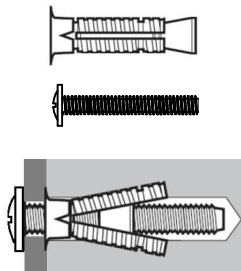
Metal Wall plug
